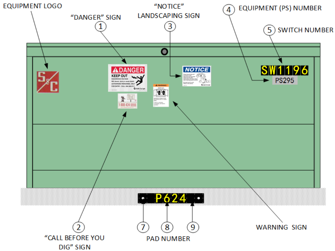
Figure 4.4h. Manual Vista Switch, Front View
