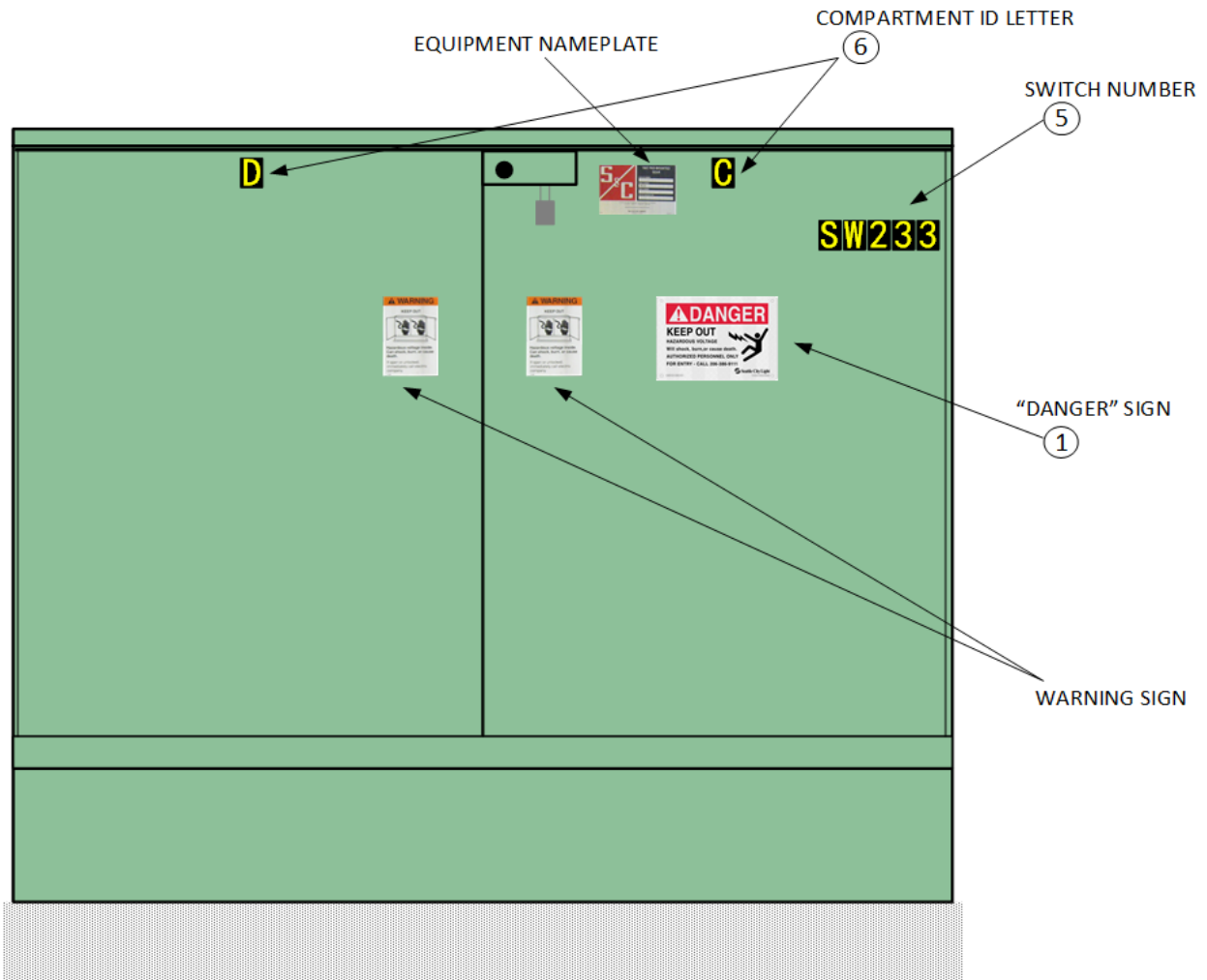
Figure 4.2b. Four-Compartment PMH Switch, Rear View
