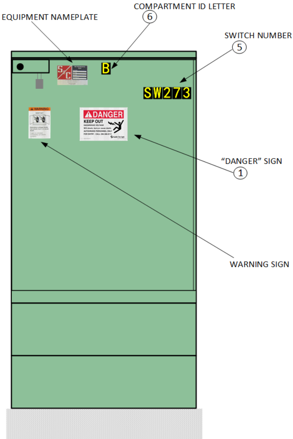
Figure 4.3b. Two-Compartment PMH Switch, Rear View
