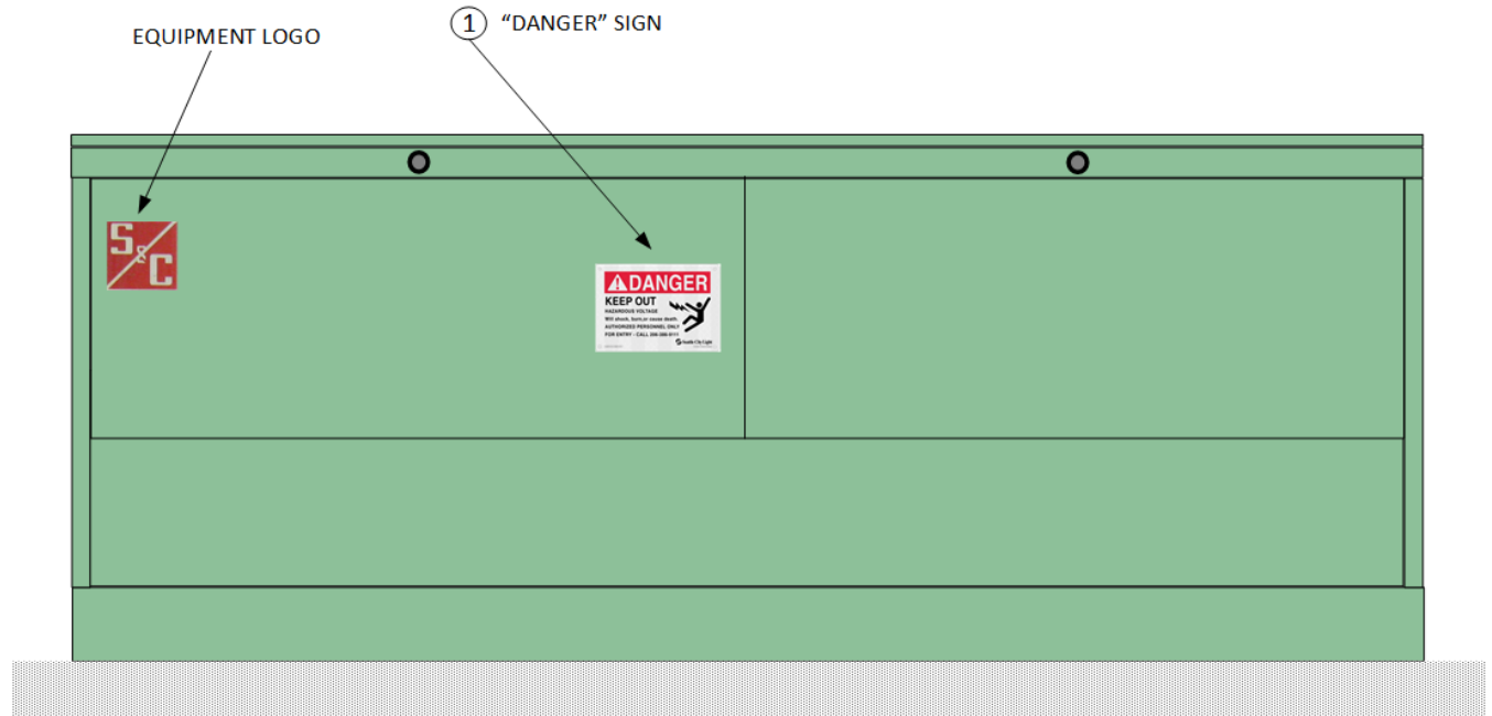
Figure 4.4f. Remote Supervisory Vista Switch LVE with Pedestal Mount, Double Swing Doors
