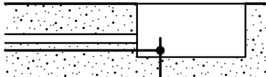
Figure 6.1. Direct buried conduits entering a single vault or handhole
