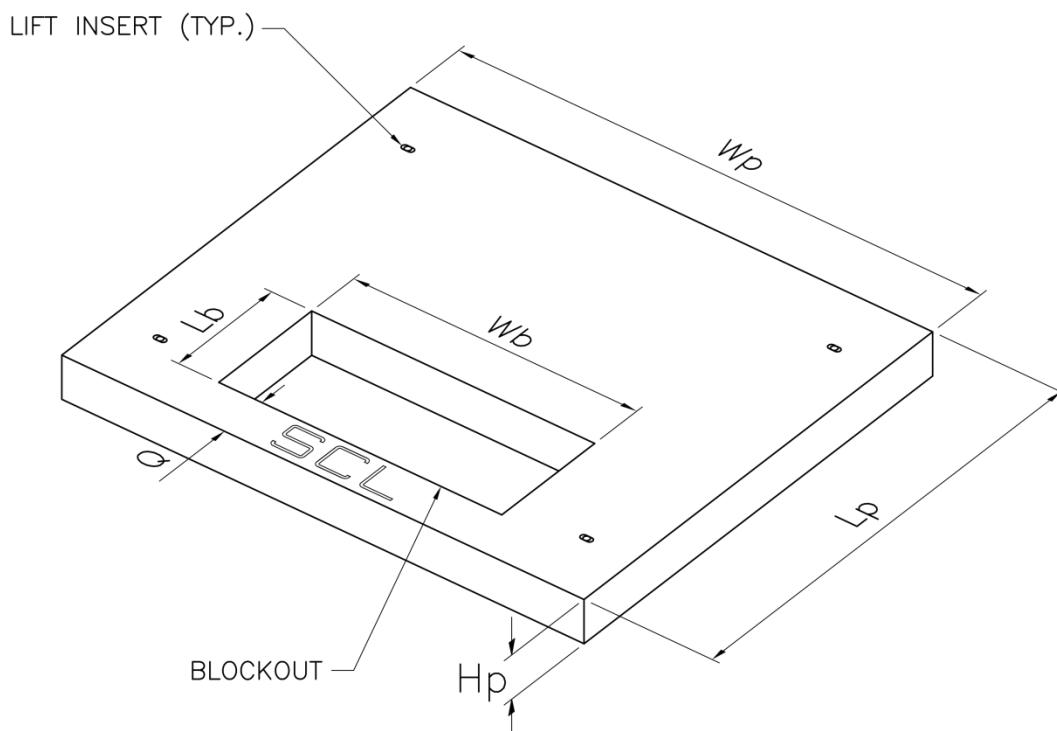
Figure 4.2a. Transformer Pad
