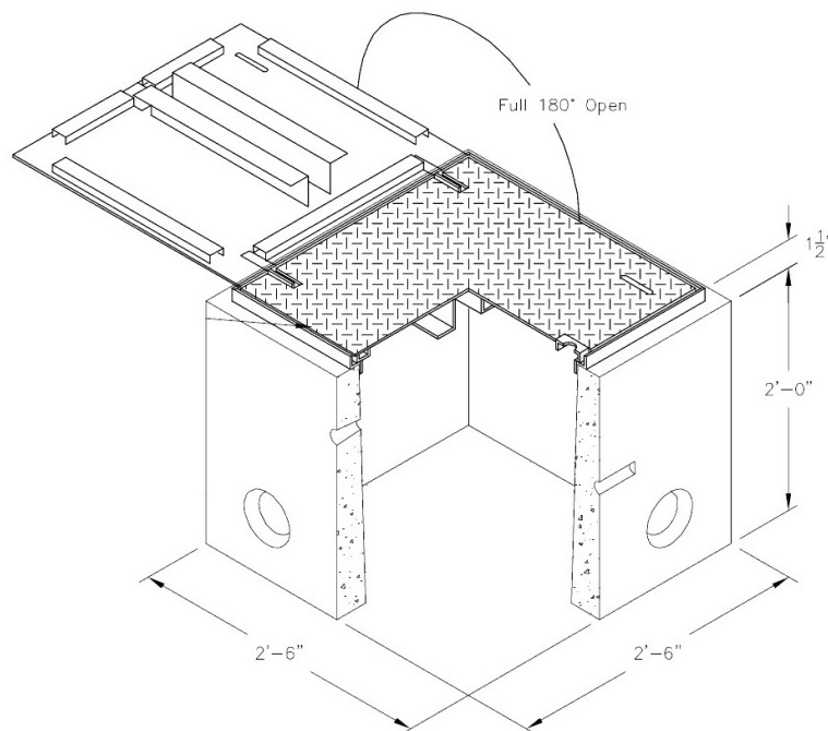
Figure 4.2. 3030 Handhole
