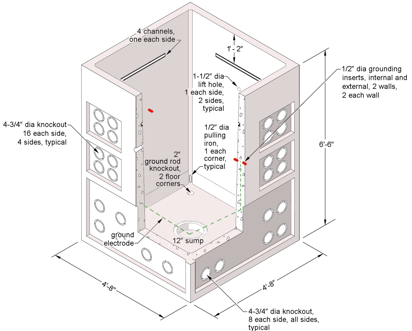
Figure 4.2. Base
