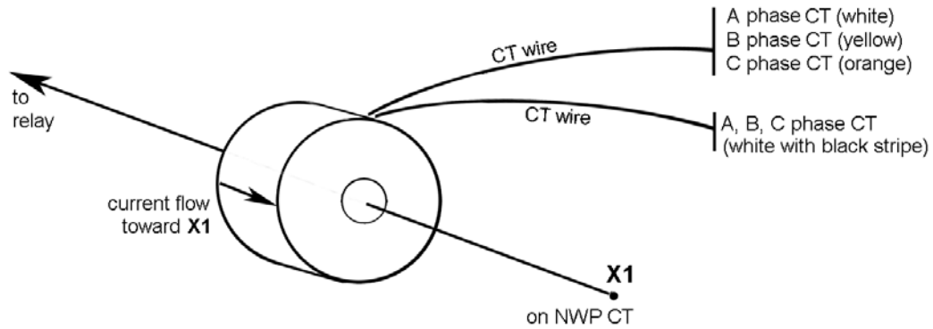
Diagram W5 – NCS CT orientation (3 CT representation)
