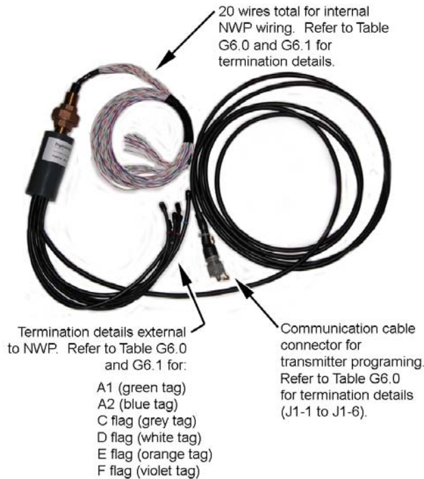
Photo G6 – NCS Auxiliary Cable Harness Model No. DG-210
