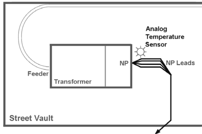
Diagram S2.1 Street Transformer Vaults
