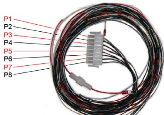
Photo W3 – NCS Wire Harness Model No. DG-200
