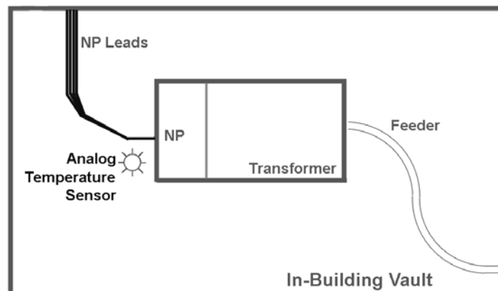
Diagram S2.2 New, In-Building Vault - One Transformer
