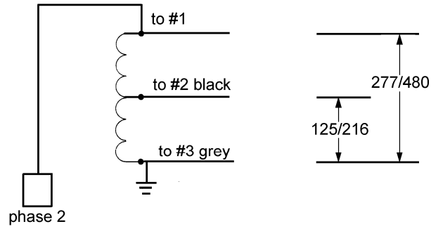
Diagram W9 – Autotransformer Wire Connection
