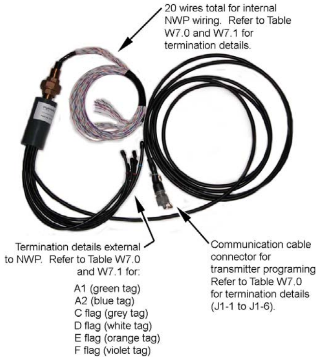
Photo W7 – NCS Auxiliary Cable Harness Model No. DG-210
