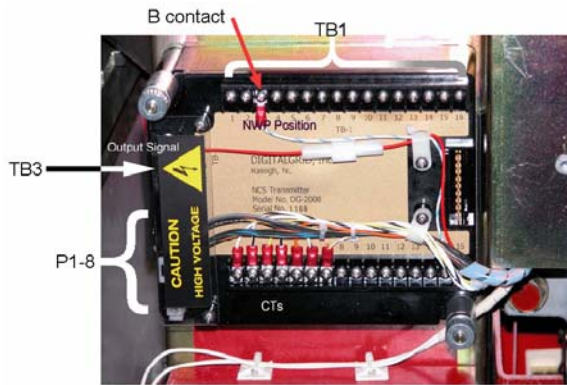
Photo G1 – Wired NCS Transmitter Model No. DG-2000
