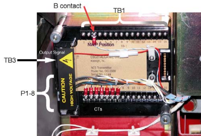
Photo W1 – Wired NCS Transmitter, Model No. DG-2000
