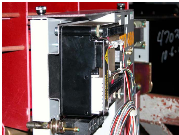
Photo W6 – NCS Transmitter With NCS Transmitter Bracket Part No. DG-5003 in NWP
