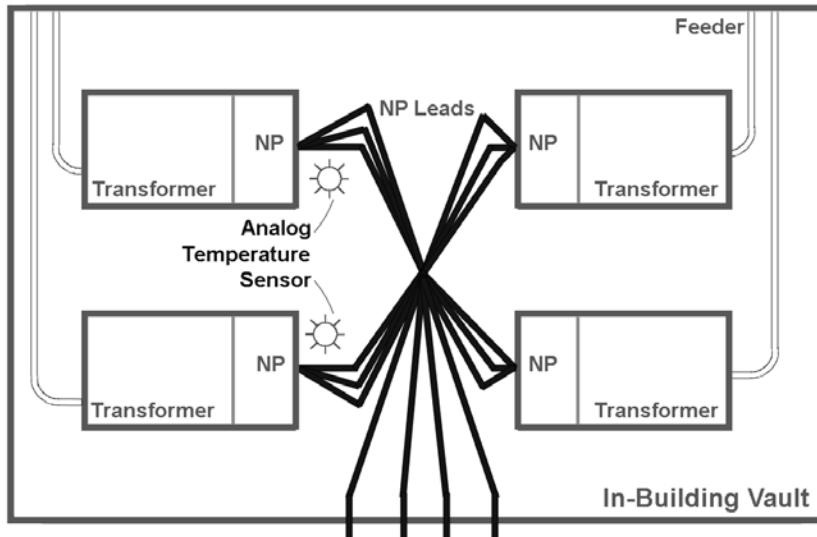
Diagram S2.3 In-Building Vault - More than One Transformer
