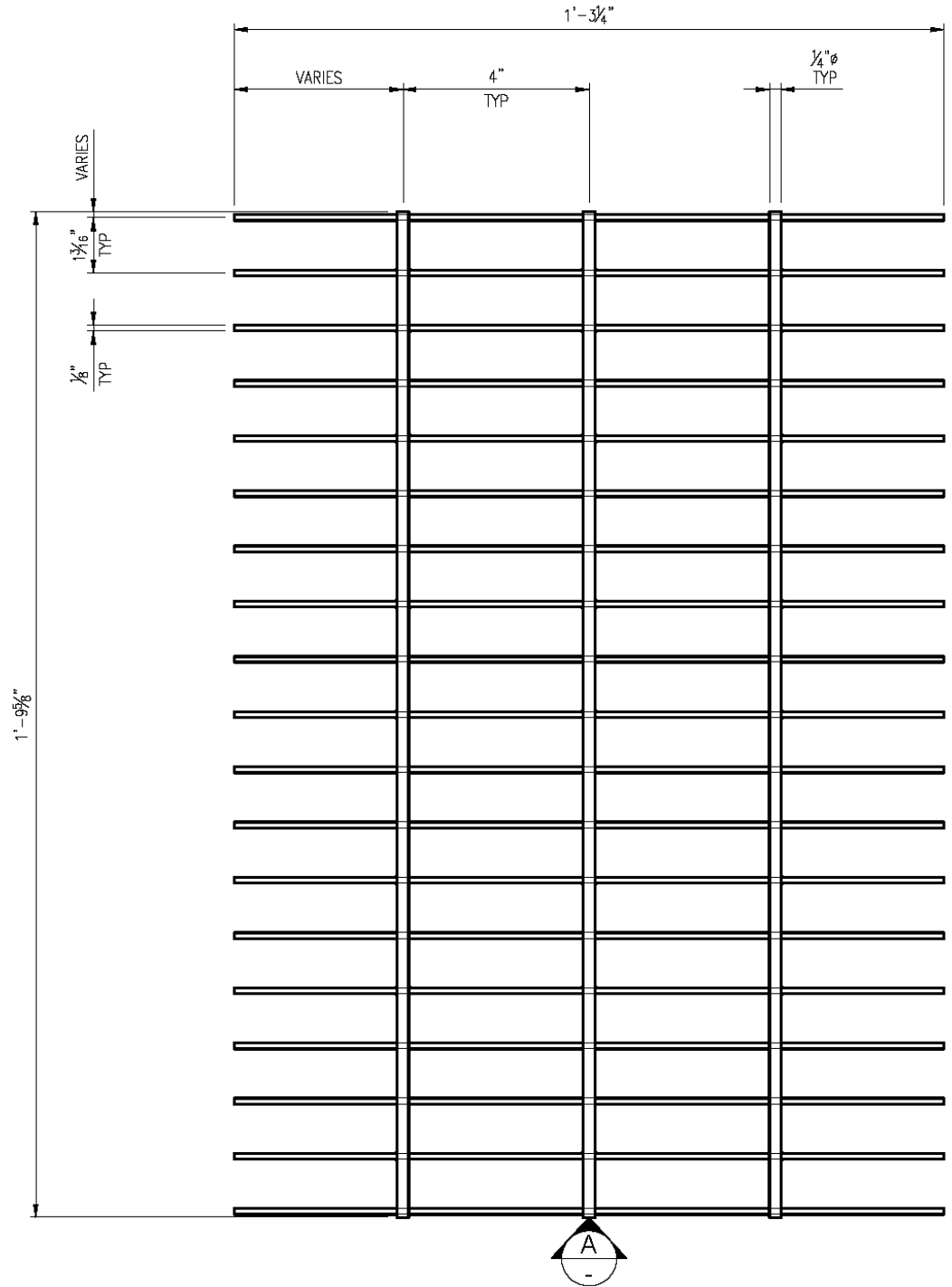
Figure 4. Sump Pump Grate Dimensions
