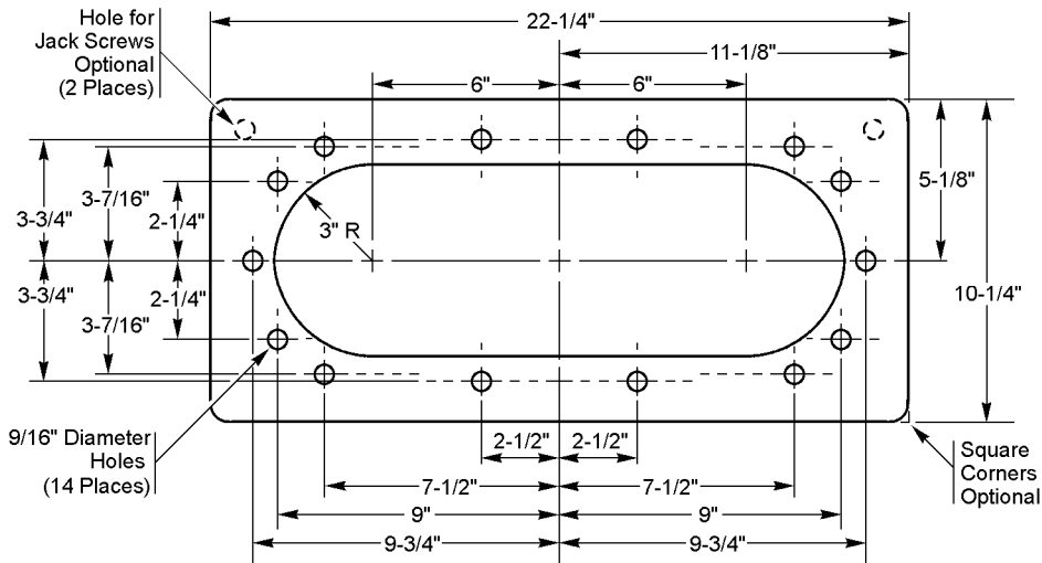
Gasket for 800 through 1875 AMP Protectors Stock No. 686798
