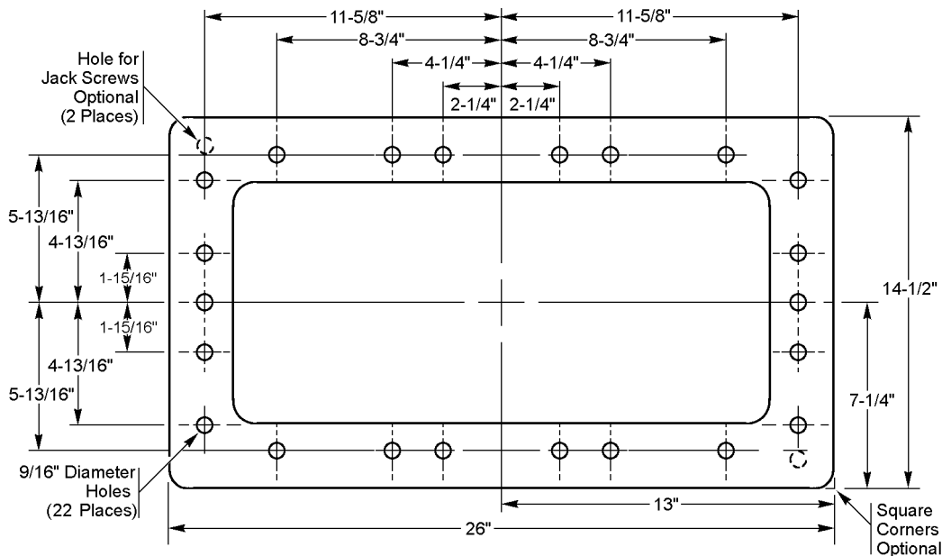
Gasket for 2500 through 3500 AMP Protectors Stock No. 686799
