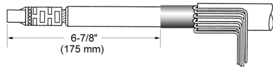
Figure 4, Cutback Length
