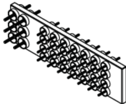
Figure 9.10. Bus Bar Section, 28 Cable Positions
