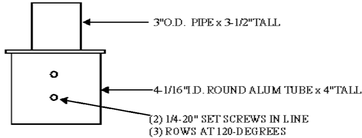
Figure 4a. Adapter, Side View
