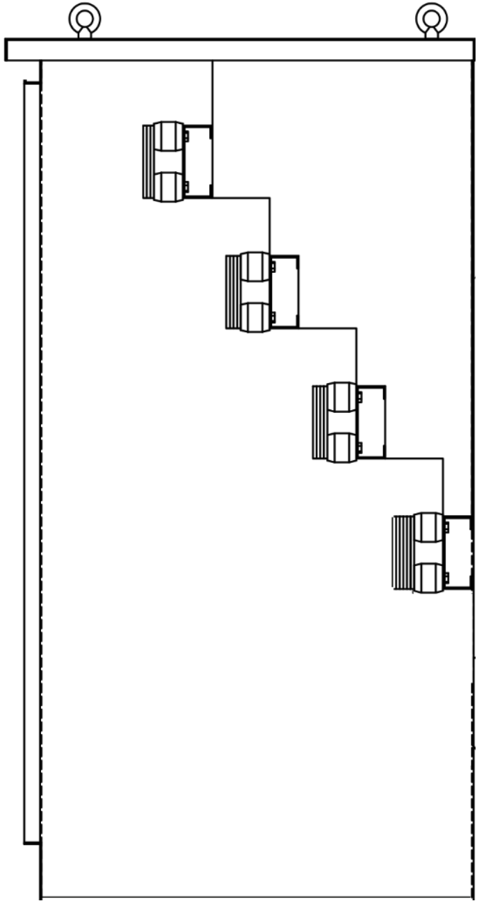
Figure 3.2b. Bus Bars, Tiered, Side View
