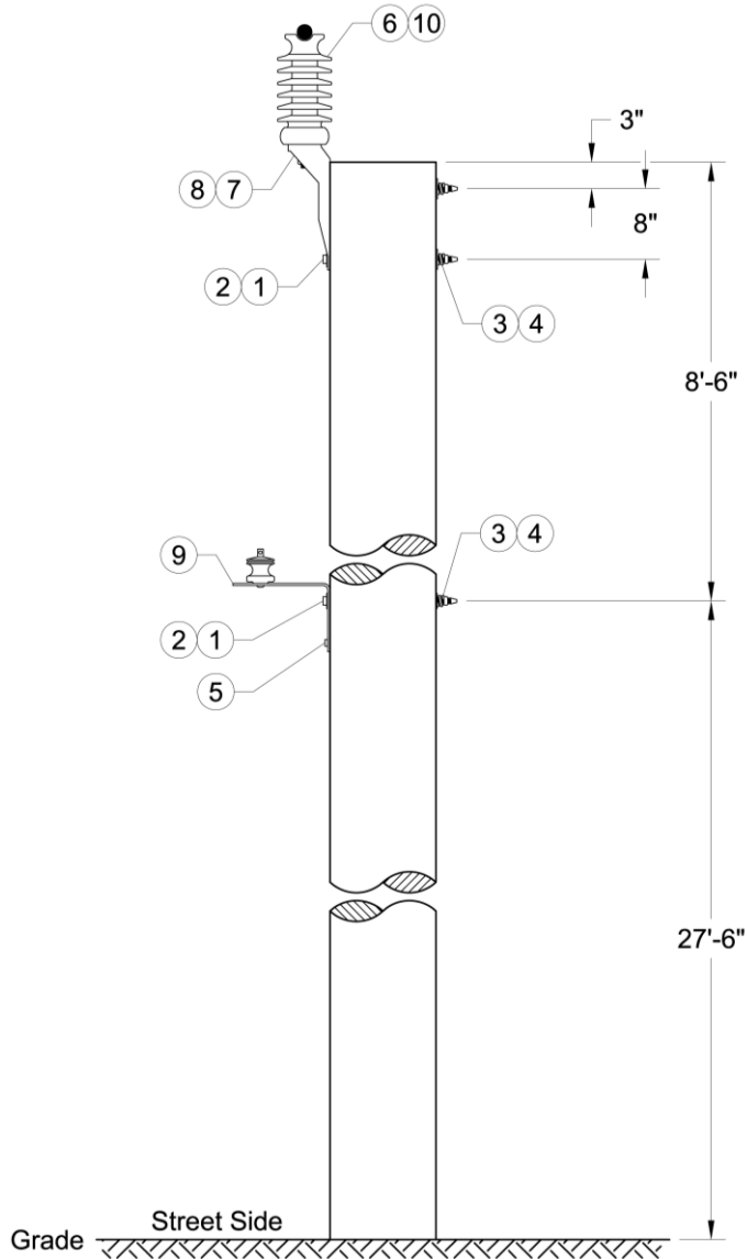
Figure 3b. Single-Phase Tangent Pole Top Assembly for View Areas
