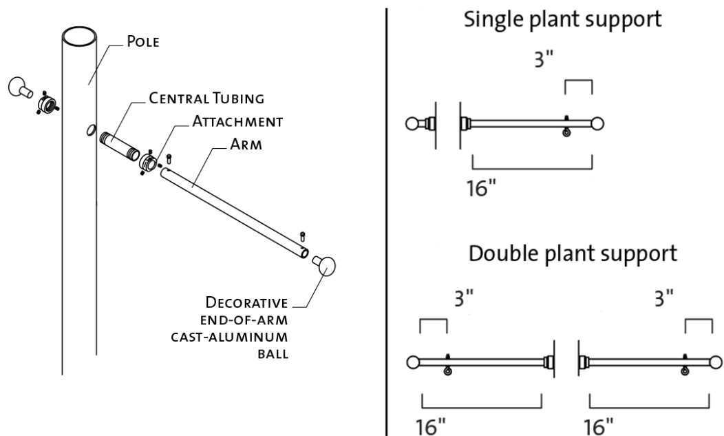
Figure 3. Planter Support Arms
