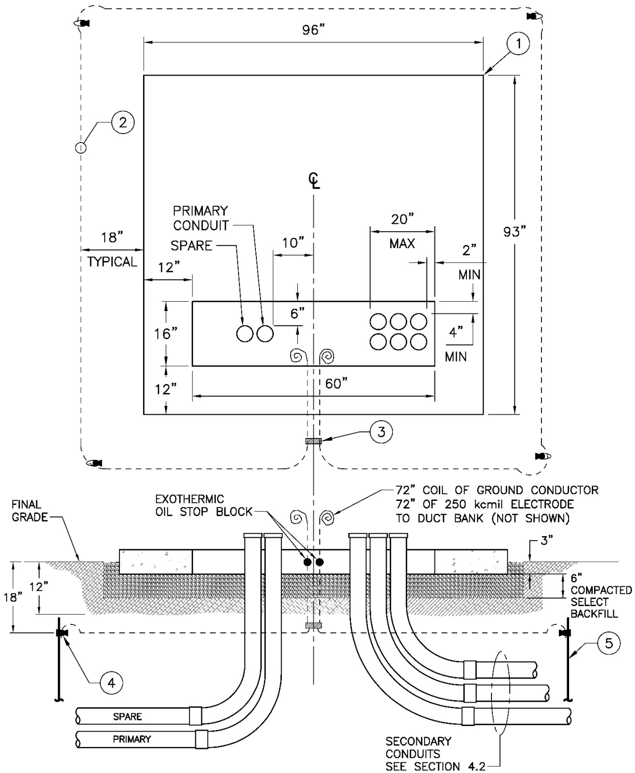
Figure 5b. Small Three-Phase Transformer Pad Requirements
