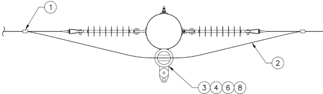
Figure 3e. Single-Phase Single-Gain Double Deadend 0°–100° Head Pin Jumper, Top View
