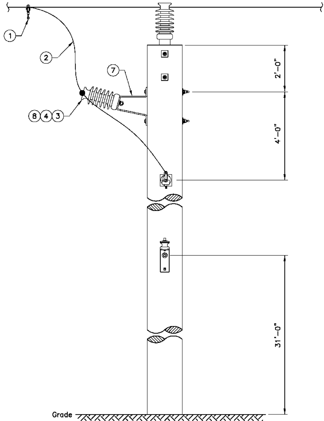
Figure 3I. Single-Phase Multi-Gain Tangent to Deadend Jumper, Side View
