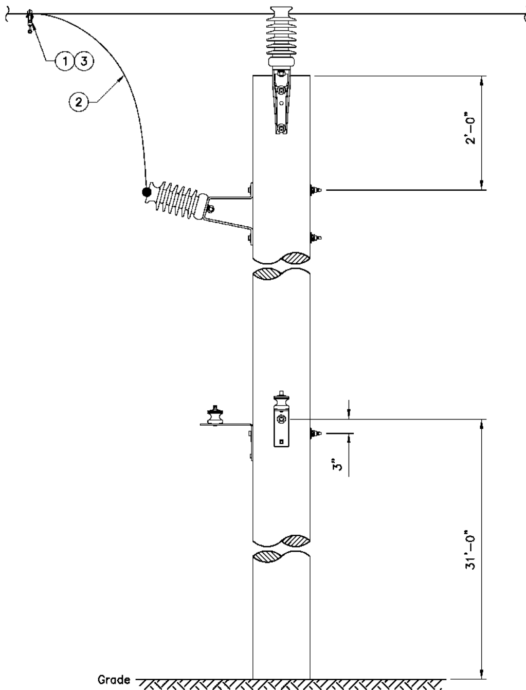
Figure 3p. Single-Phase Multi-Gain Tangent to Tangent Jumper, Side View
