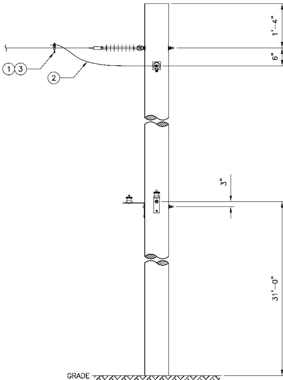
Figure 3n. Single-Phase Multi-Gain 100°-180° Jumper, Side View
