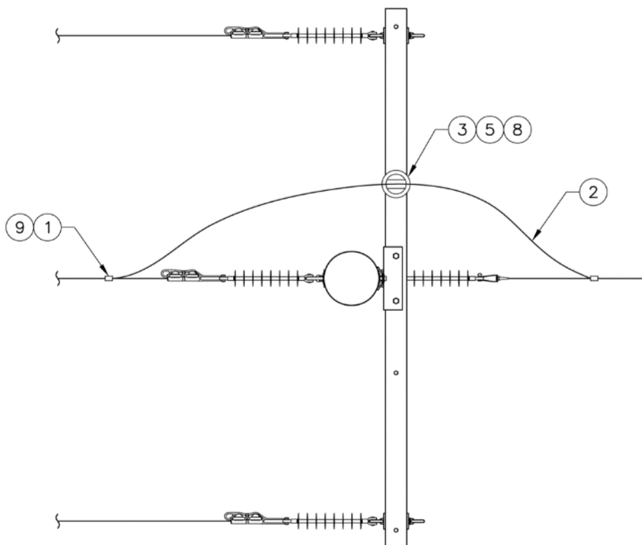
Figure 3a. Single-Phase Double Deadend 0°–60° Crossarm Jumper, Top View
