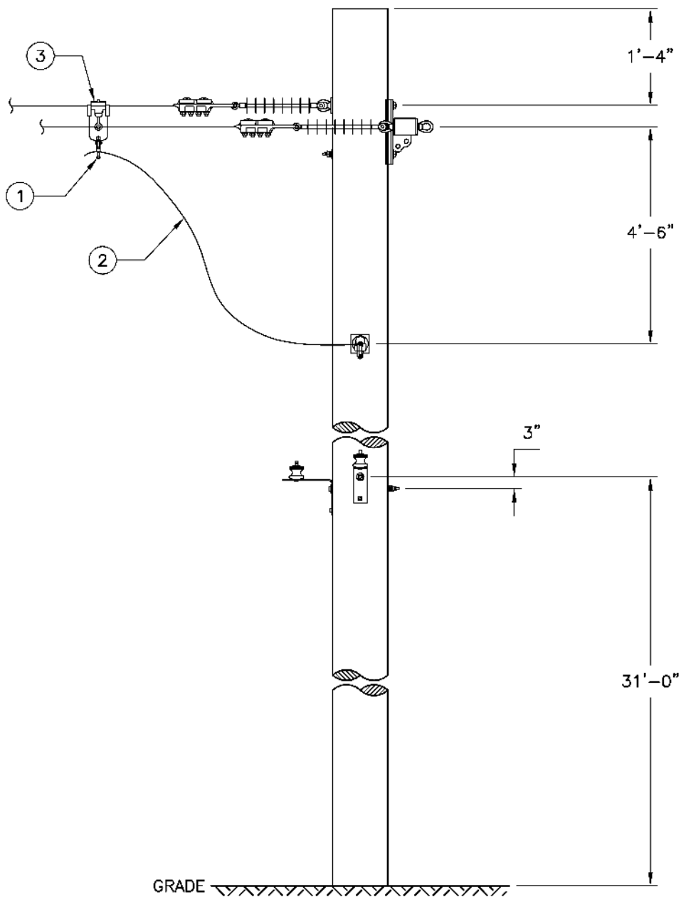
Figure 3d. Single-Phase Double Deadend 60°–180° Crossarm Jumper, Side View
