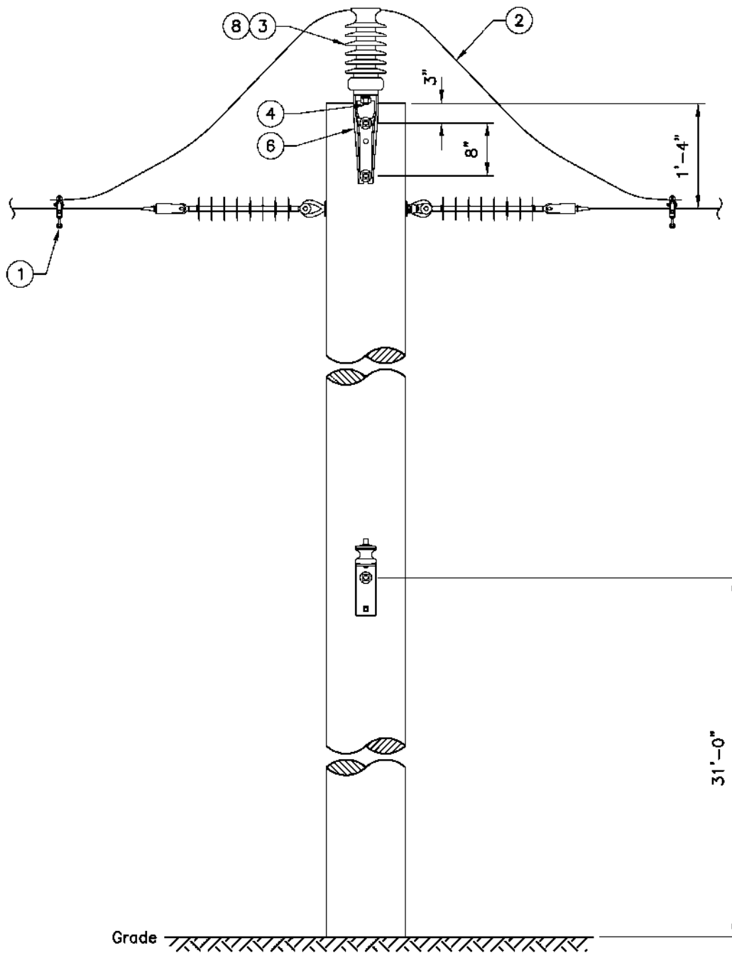
Figure 3f. Single-Phase Single-Gain Double Deadend 0°–100° Head Pin Jumper, Side View
