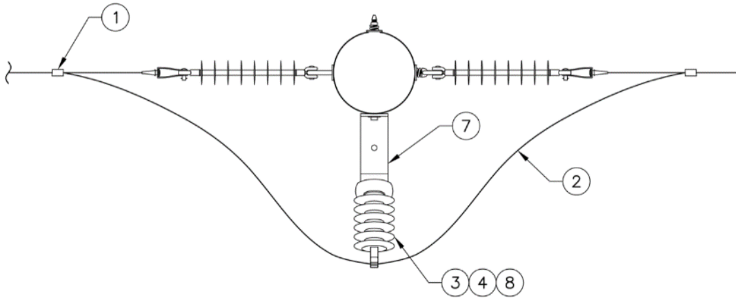
Figure 3i. Single-Phase Multi-Gain 0°-100° Deadend to Deadend Side Mount Jumper, Top View
