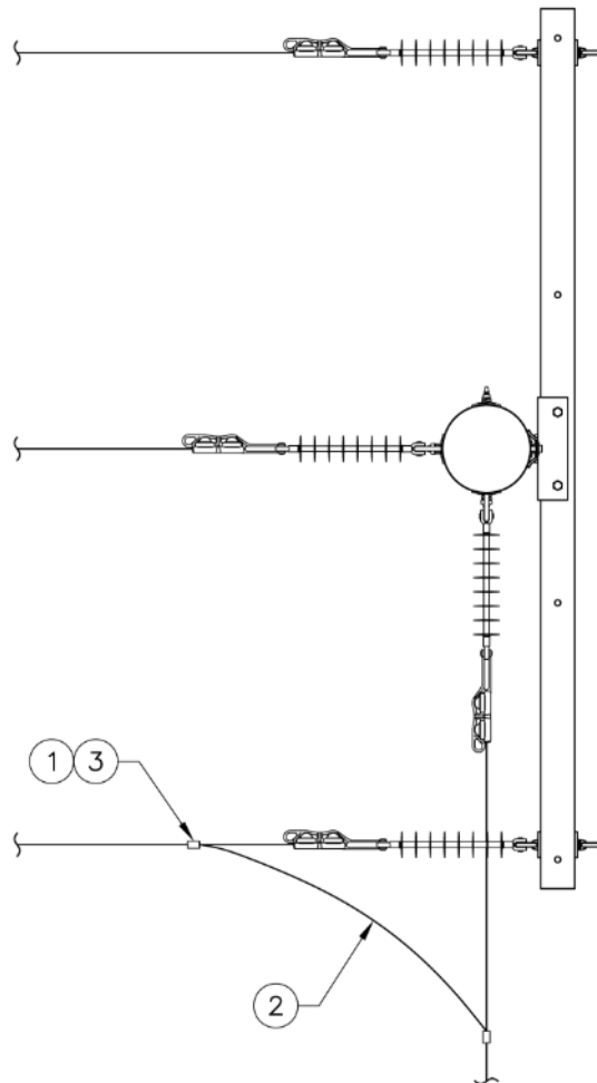
Figure 3c. Single-Phase Double Deadend 60°–180° Crossarm Jumper, Top View
