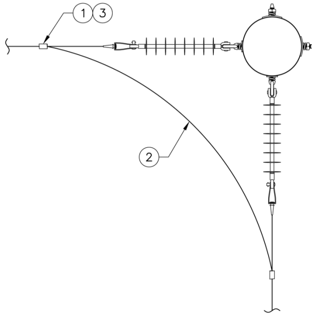
Figure 3m. Single-Phase Multi-Gain 100°-180° Jumper, Top View
