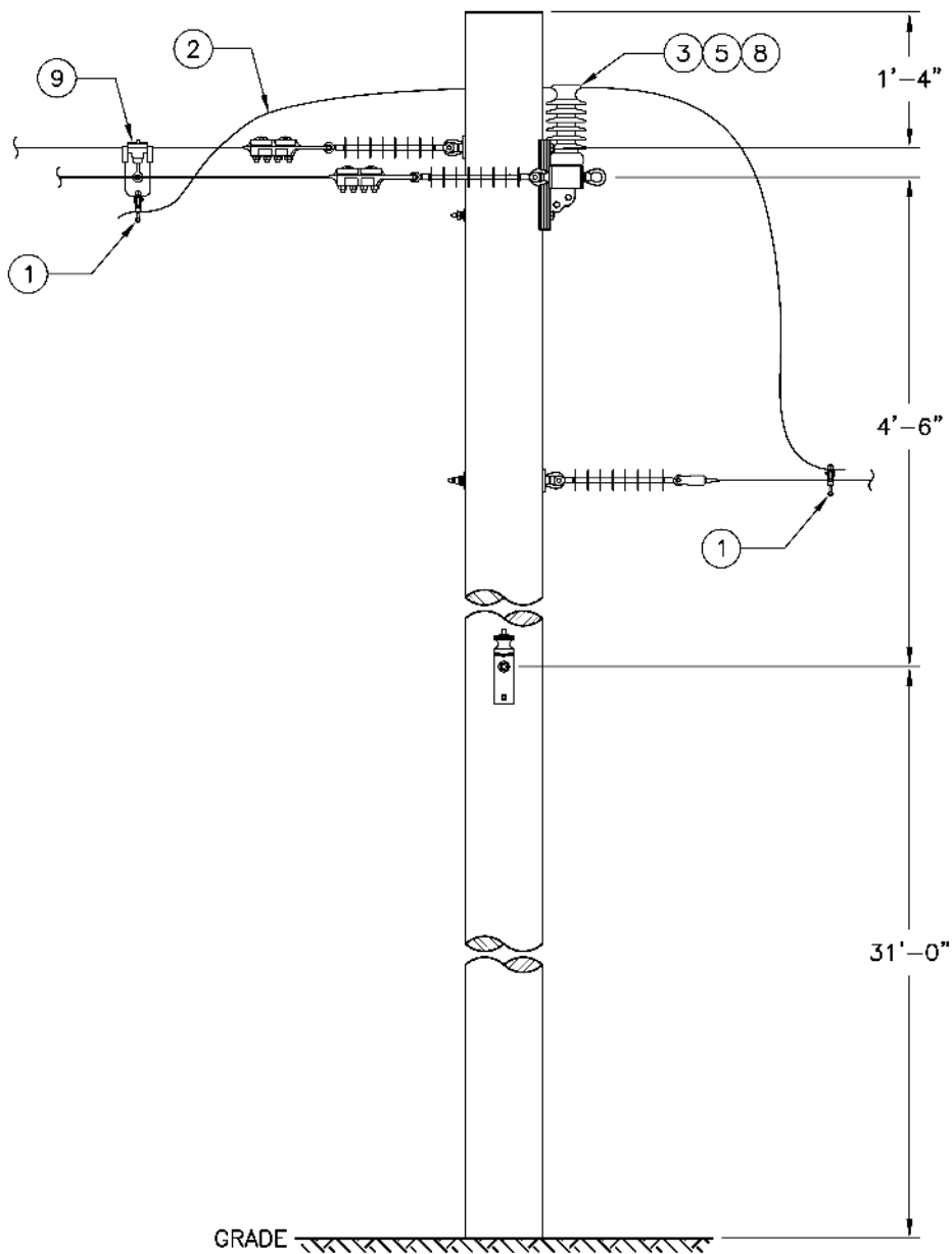
Figure 3b. Single-Phase Double Deadend 0°–60° Crossarm Jumper, Side View
