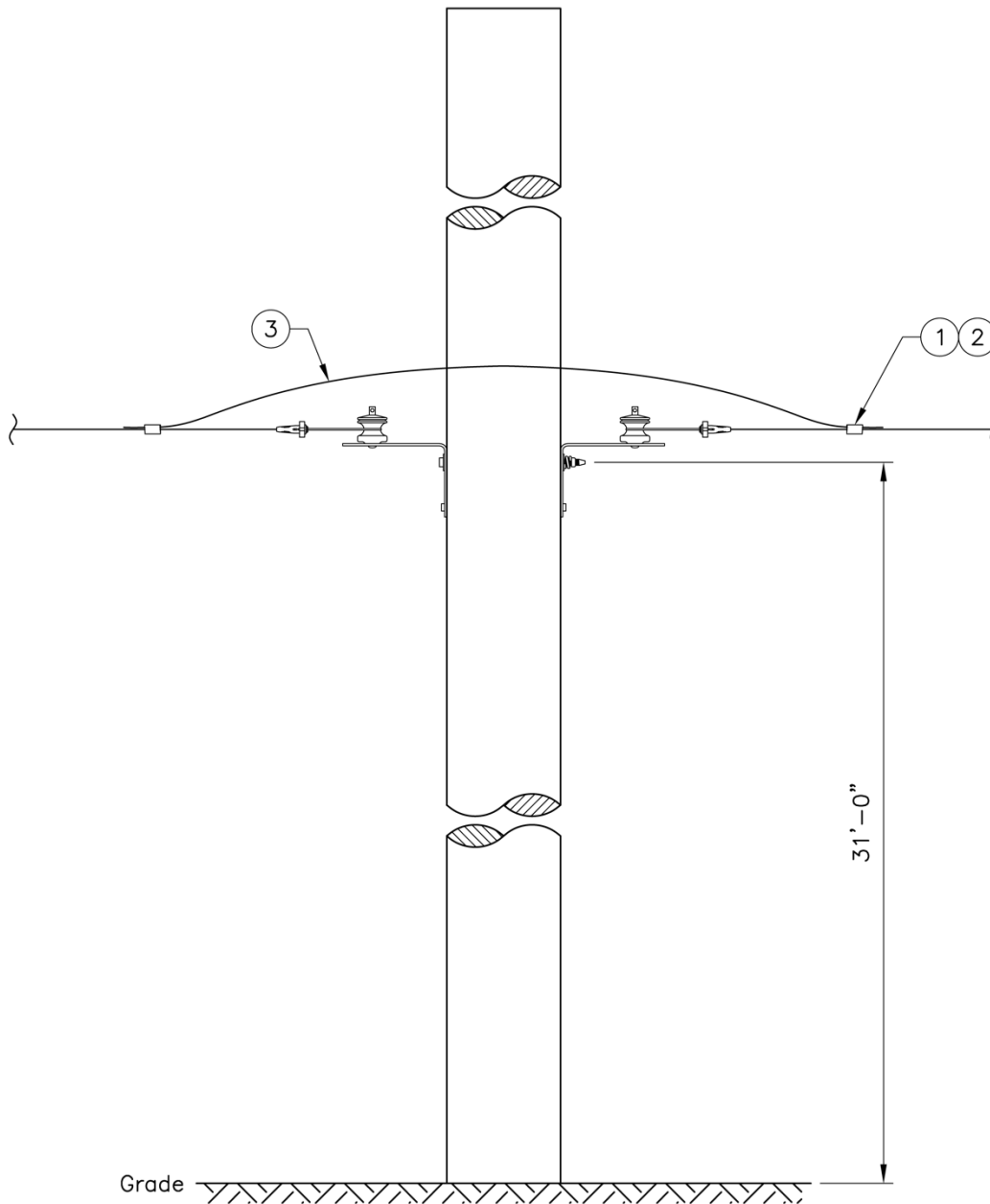
Figure 3q. Neutral Jumper, Side View
