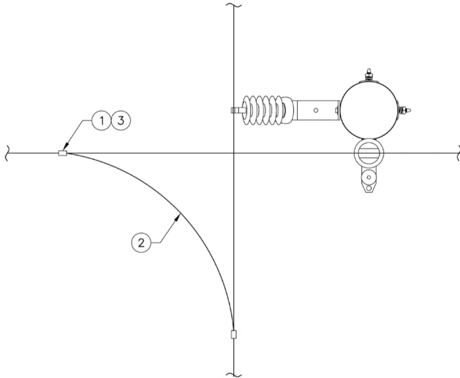
Figure 3o. Single-Phase Multi-Gain Tangent to Tangent Jumper, Top View
