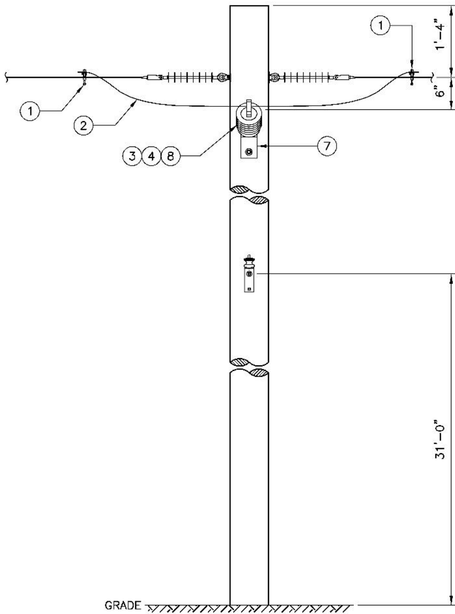
Figure 3h. Single-Phase Single-Gain Double Deadend 0°-100° Side Mount Jumper, Side View
