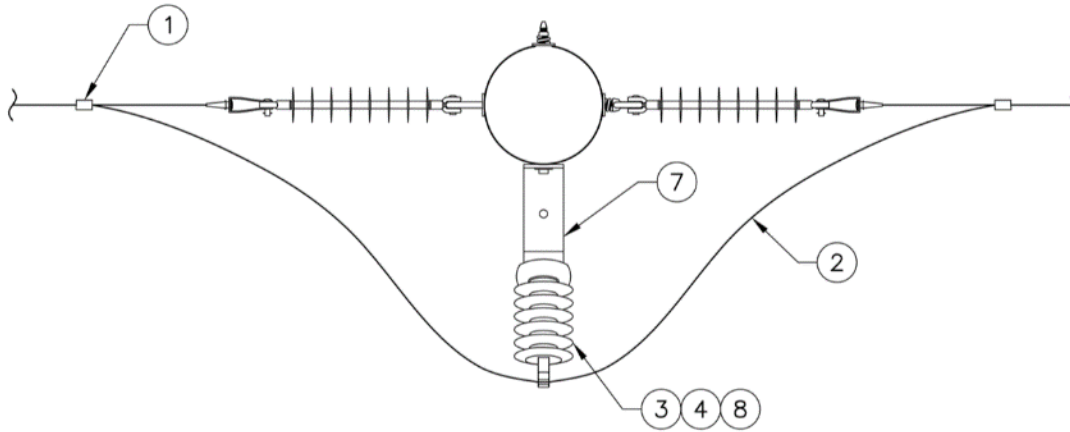
Figure 3g. Single-Phase Single-Gain Double Deadend 0°–100° Side Mount Jumper, Top View
