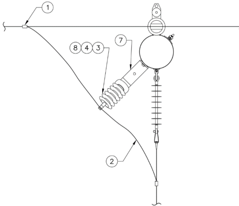
Figure 3k. Single-Phase Multi-Gain Tangent to Deadend Jumper, Top View
