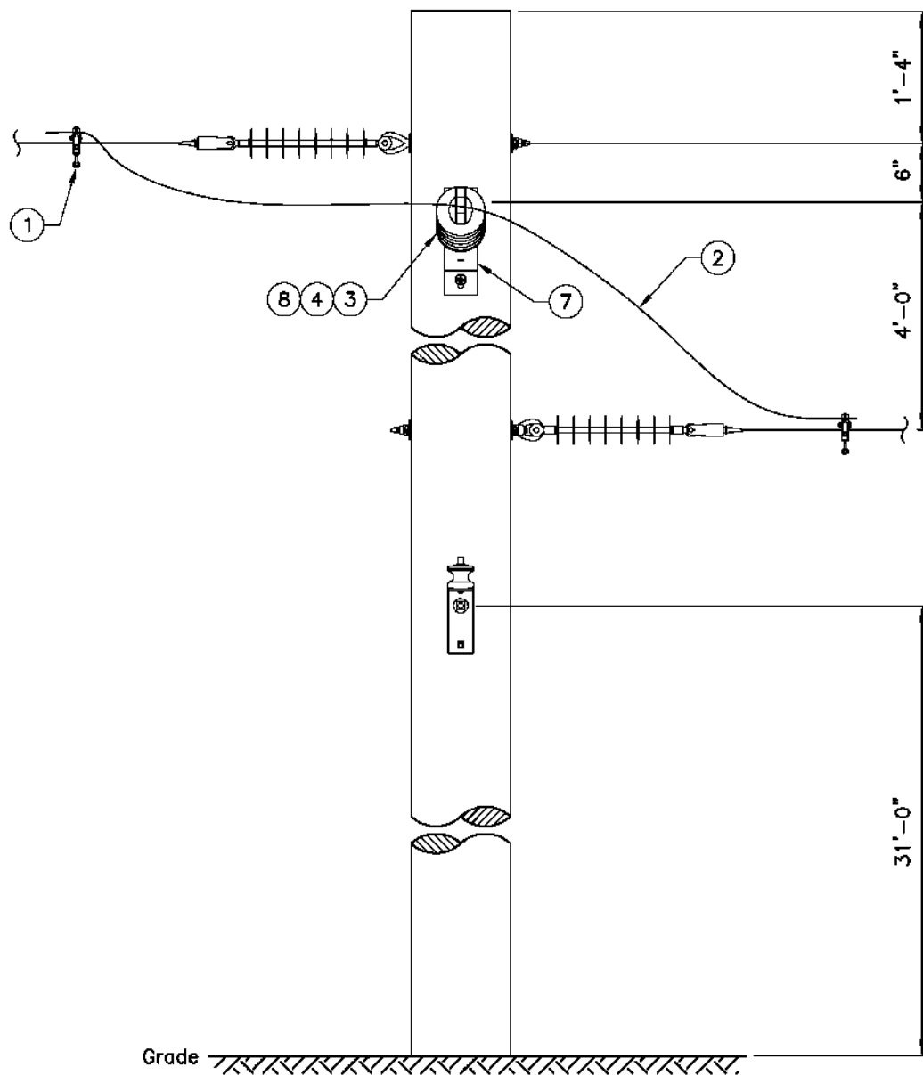
Figure 3j. Single-Phase Multi-Gain 0°-100° Deadend to Deadend Side Mount Jumper, Side View
