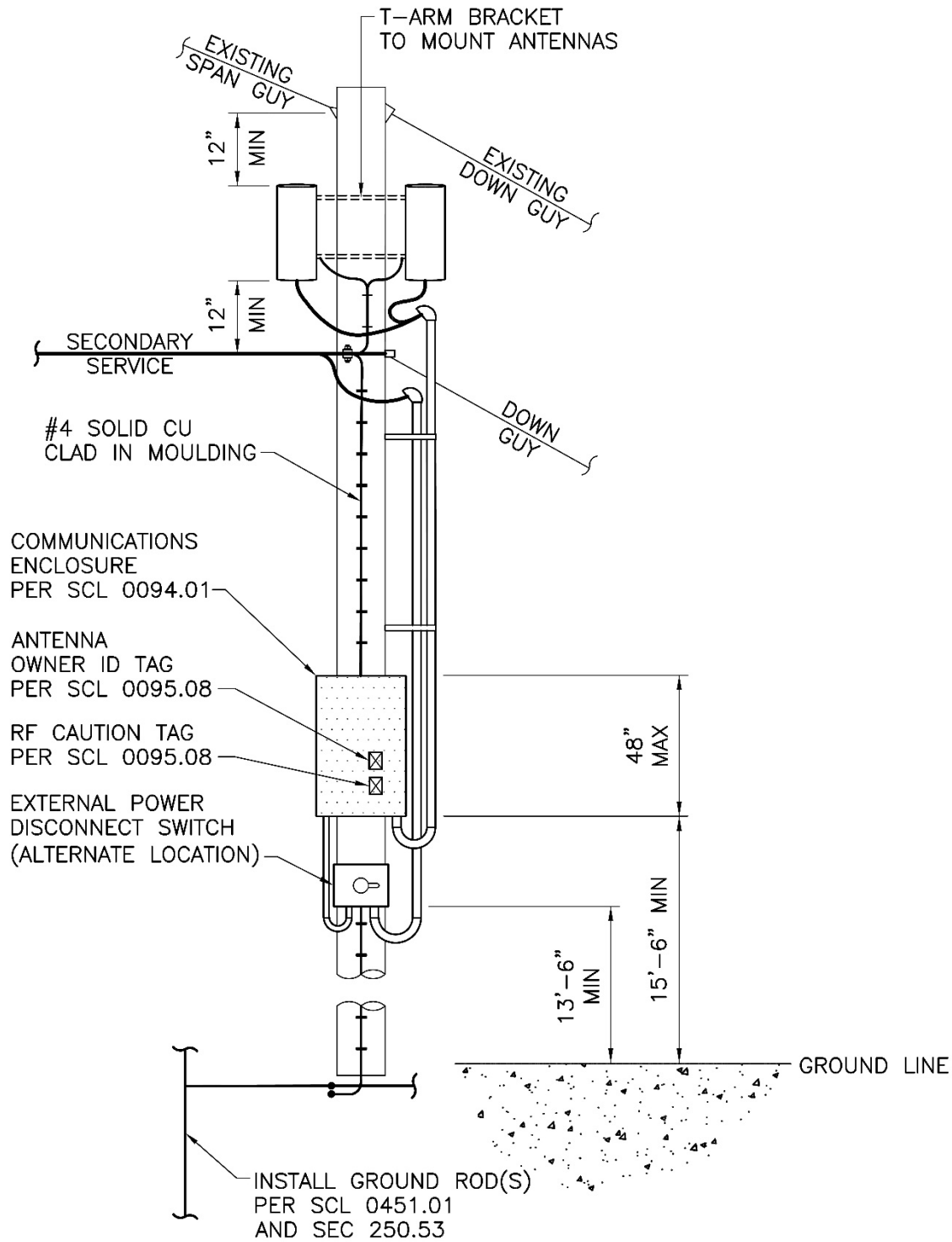
Figure 3.9b. SWF on a Guy Stub Pole
