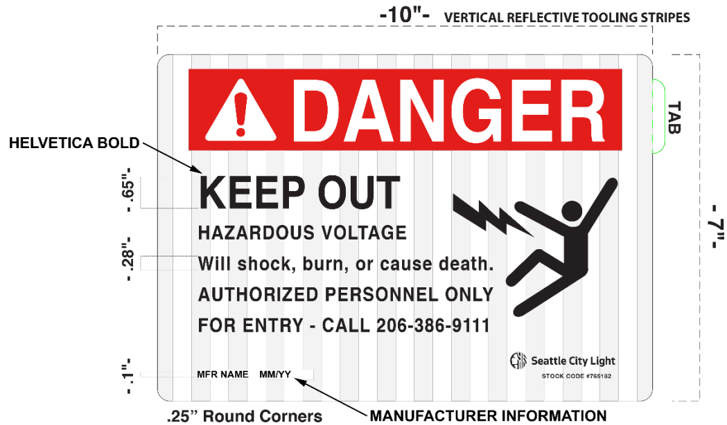
Figure 4. Example Sign Layout
