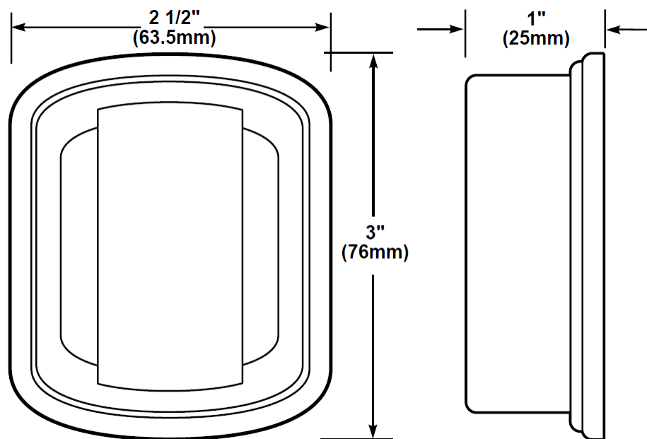
Figure 3. Buzzer Dimensions
