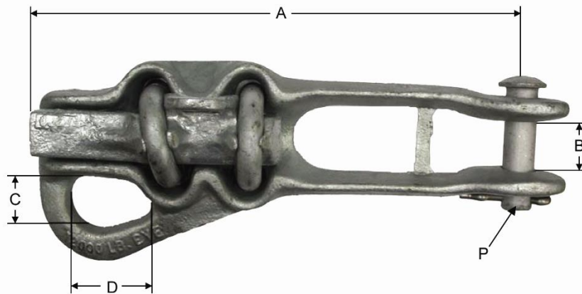
Figure 4. Clamp Dimensions
