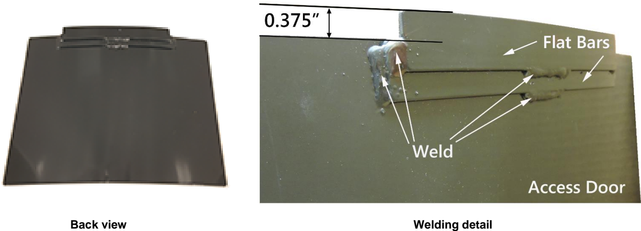
Figure 3c. Flat Bar Welding Detail
