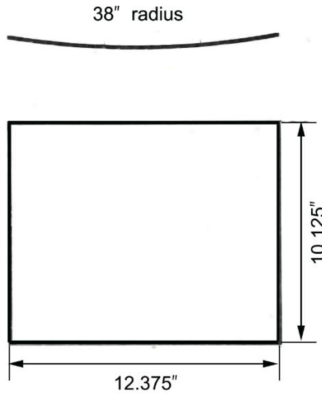
Figure 3a. Access Door Curvature and Dimensions
