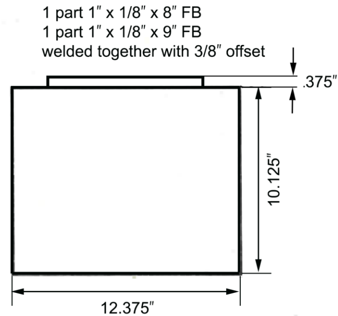
Figure 3b. Access Door with Flat Bar
