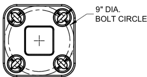
Figure 4.5. Anchor Base Detail
