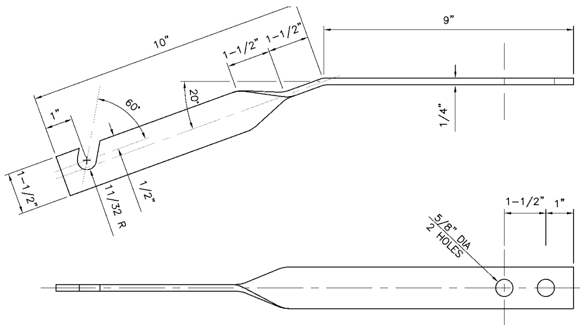
Figure 4. Reinforcing Strap Design and Dimensions
