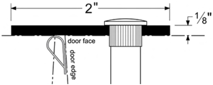
Figure 5.2.4. Astragal
