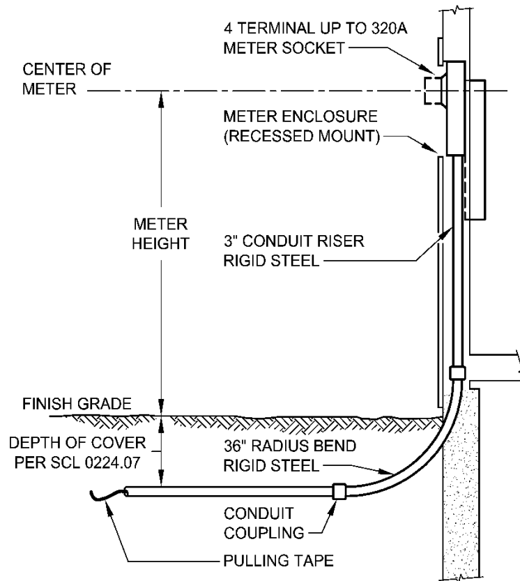
Figure 4.4.2. Recessed-Mount Meter Installation
