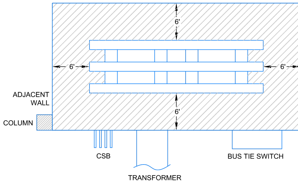
Figure 3.5b. IWCB Working Space, Plan View
