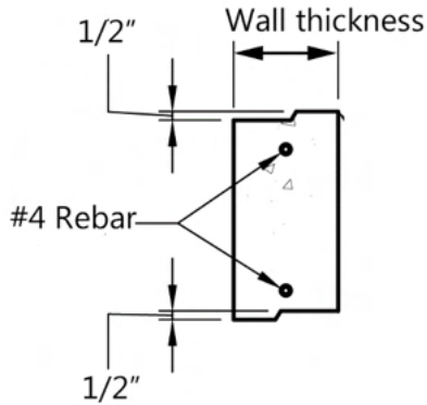
Figure 3.1b. Keyway Detail
