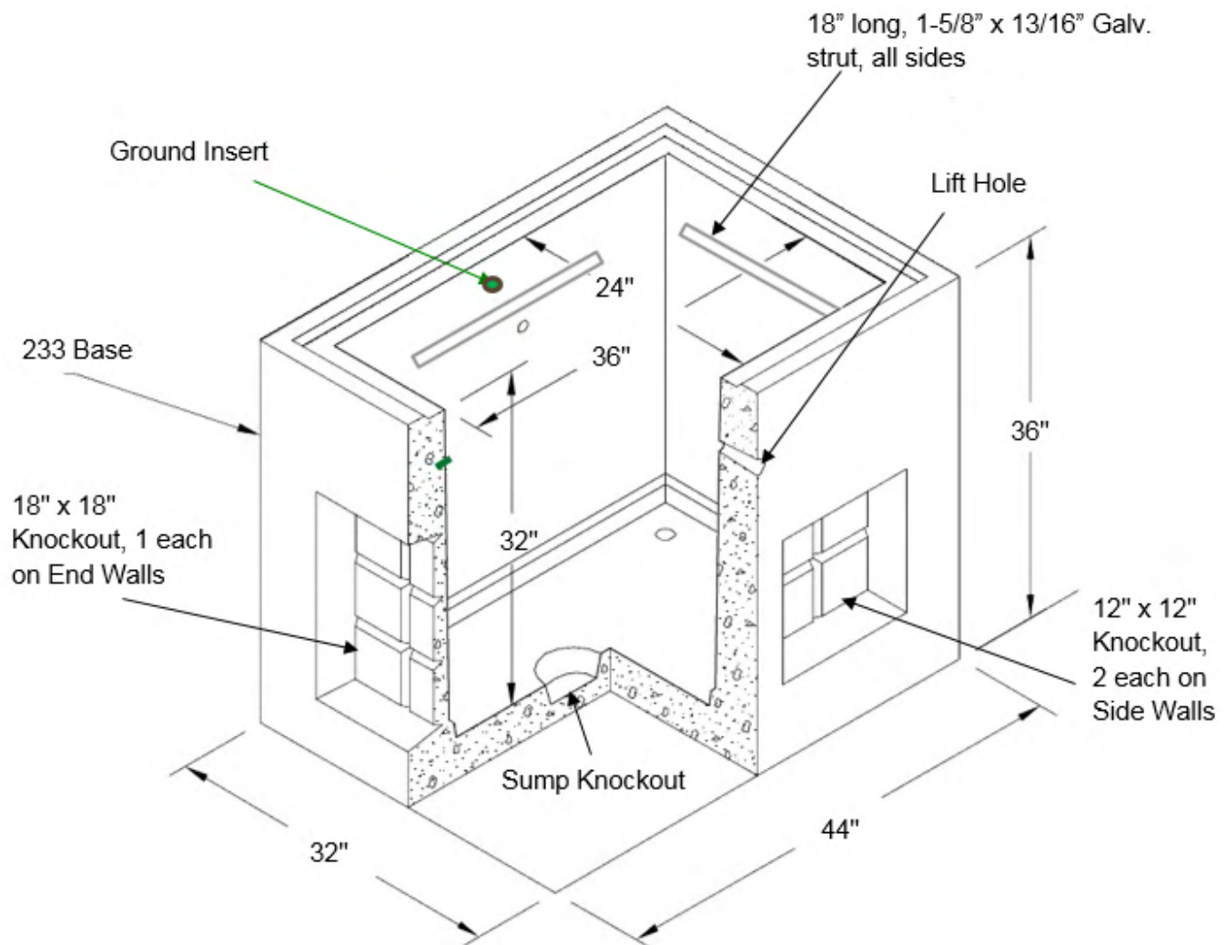
Figure 4.2. 233 Handhole Base
