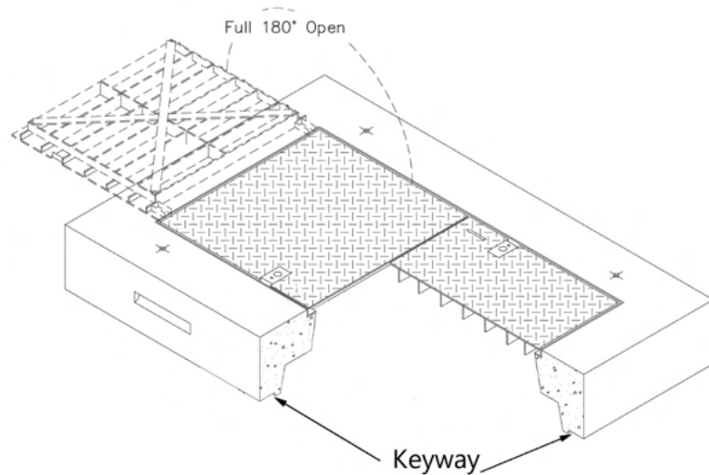
Figure 3.4. Cover With Two Hatches
