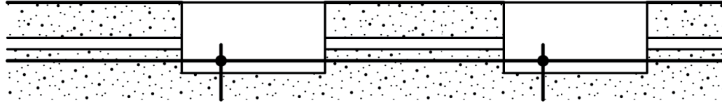
Figure 6.2. Direct buried conduits entering a series of vaults or handholes
