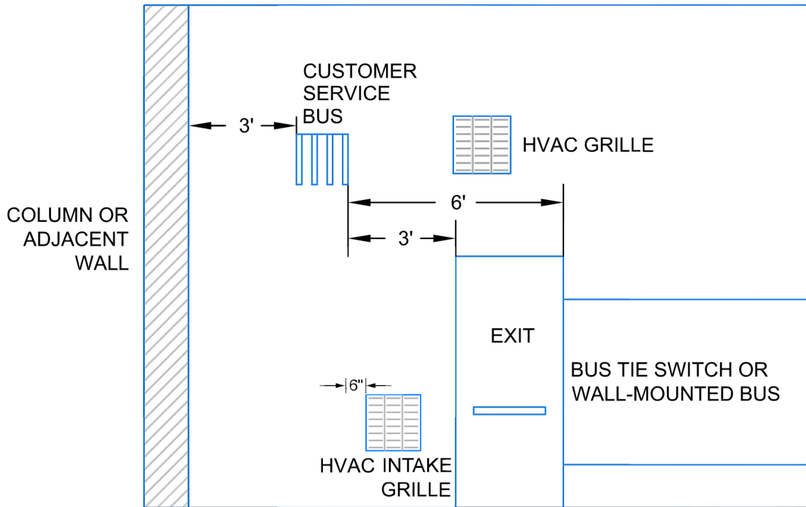
Figure 3.3c. CSB Working Space, Elevation
