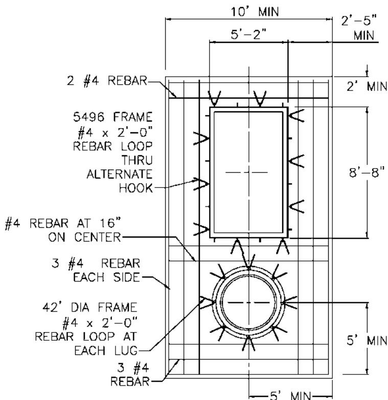
Figure 3e. Round Access and 5496 Hatch
