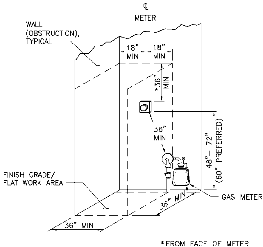
Figure 4.3b. Recessed-Mount Meter Additional Clearance Requirements
