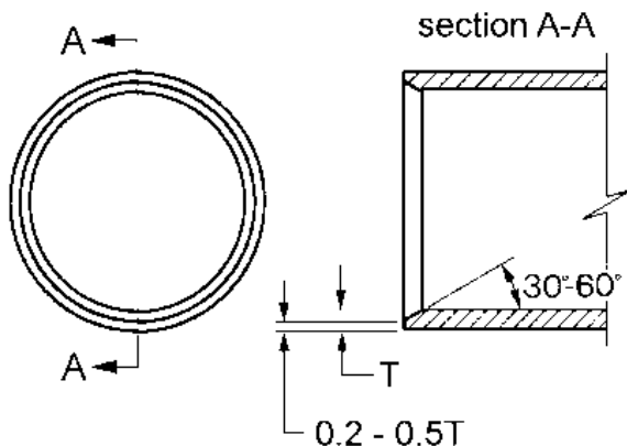
Figure 4.1. Chamfer Detail
