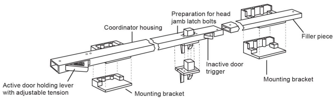
Figure 5.2.5. Door Coordinator
