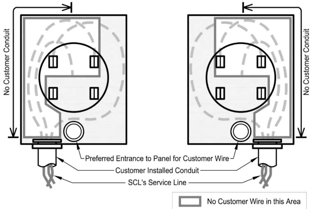
Figure 4.5. Wiring and Conduit Termination into the Enclosure
