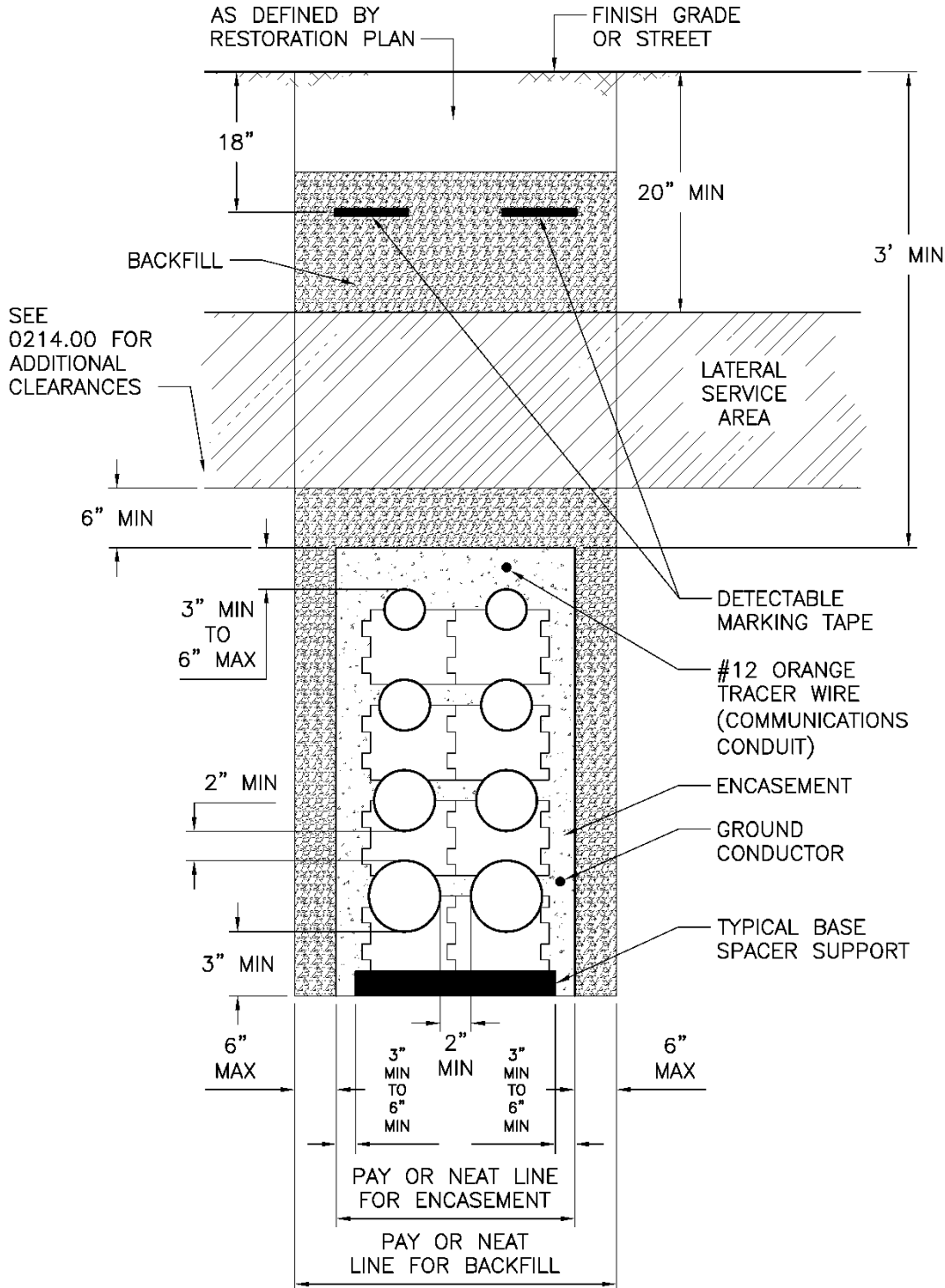
Figure 4.3a. Primary Duct Bank, End View
