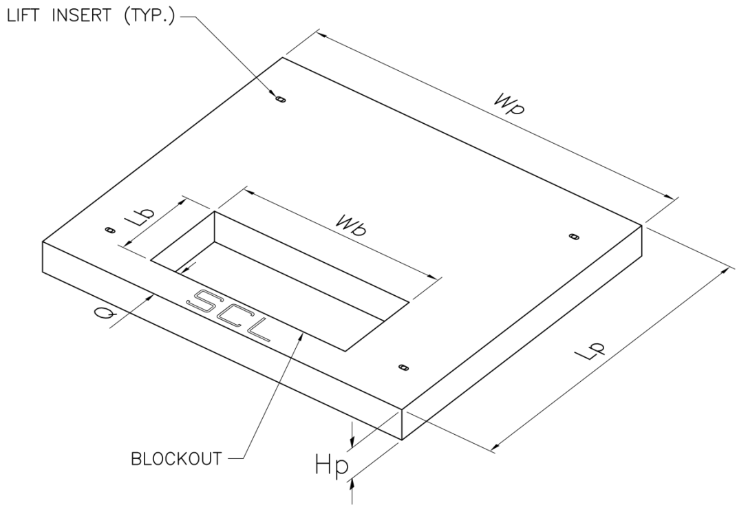
Figure 4.2a. Transformer Pad
