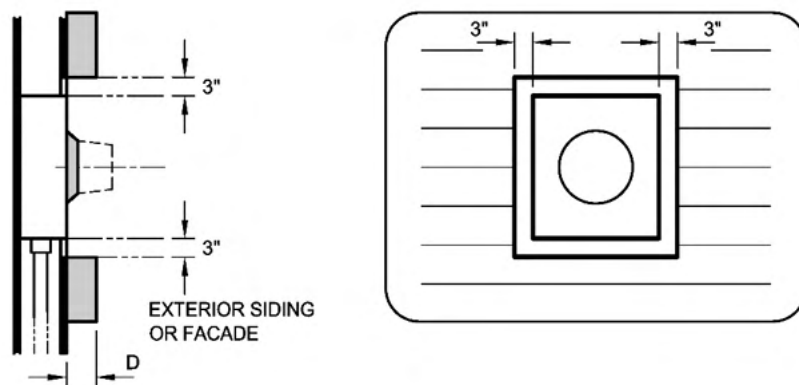
Figure 4.3b. Recessed-Mount Meter Additional Clearance Requirements
