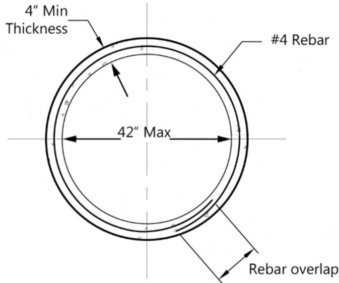
Figure 3.2. Round Riser
