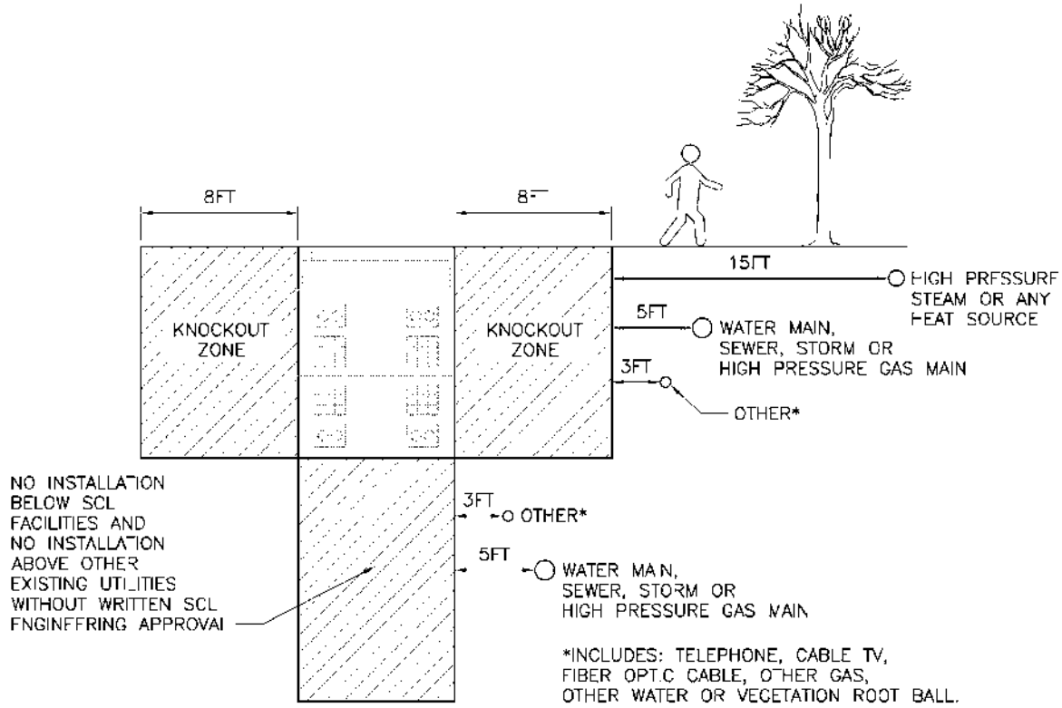
Figure 5b. Minimum Horizontal Clearance, Elevation, Side View
