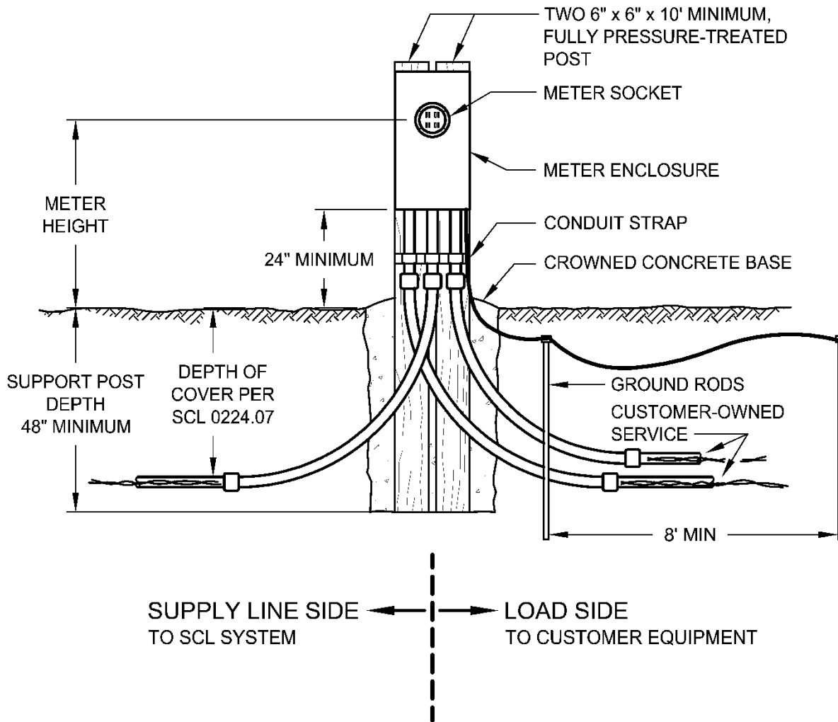
Figure 4.6.2. Pedestal-Mount Meter, 320 A
