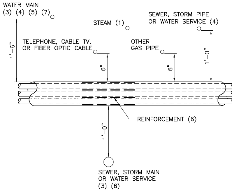
Figure 6c. Minimum Vertical Clearance, Elevation View
